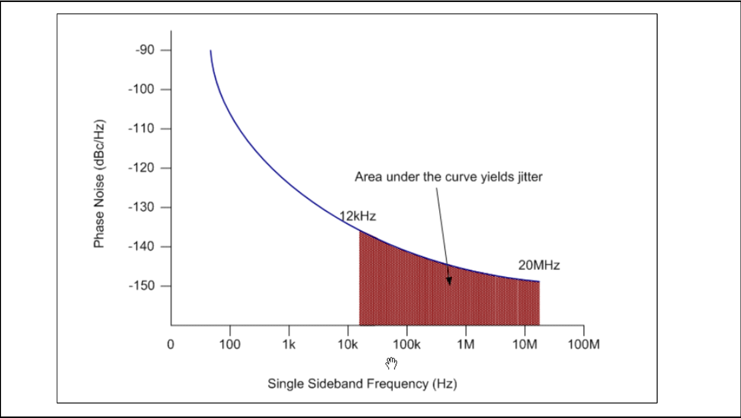
Figure 8. Phase Noise Plot of a 311MHz Oscillator (from Thomas Fischer TI). Offset (modulation) Frequencies are shown on a Logarithmic Scale.
