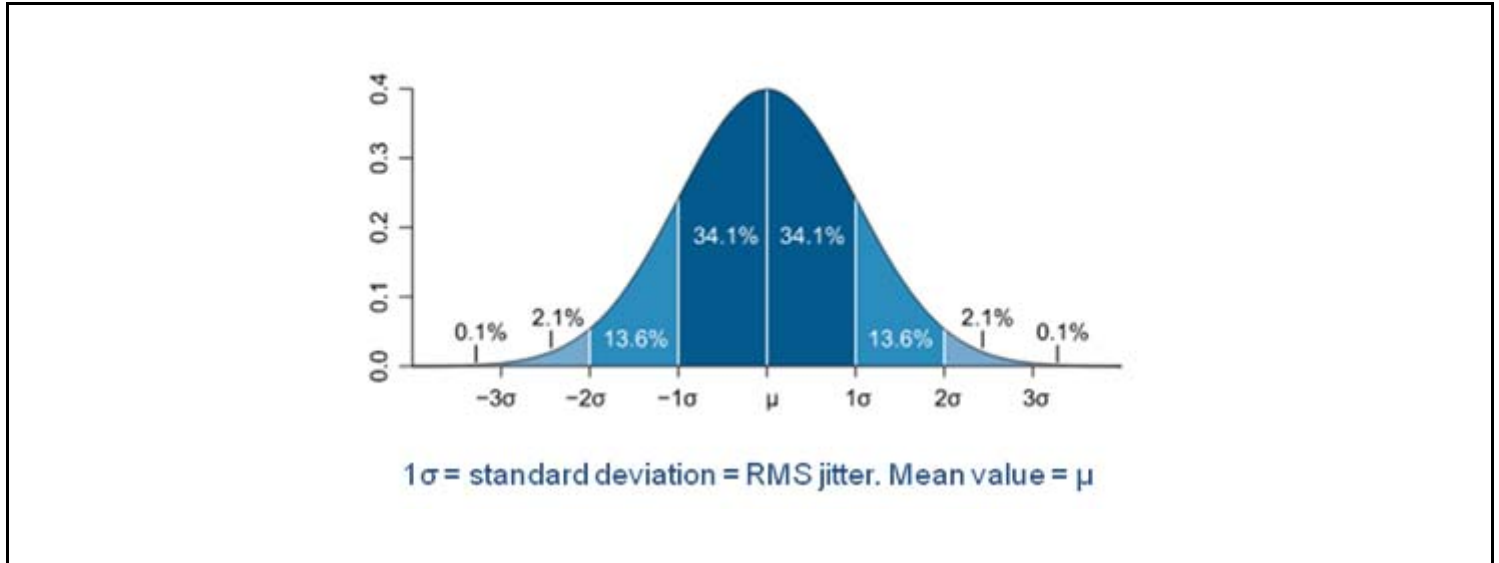
Figure 6. Gaussian (Normal) Distribution
