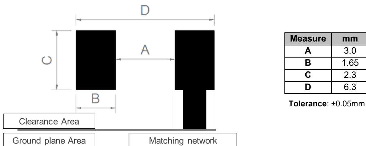
Figure 4 - Footprint dimensions for the ONE mXTEND ™ (NN02-201) antenna booster.
