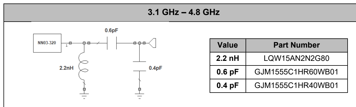
Figure 2 – Matching network implemented in the Evaluation Board (Figure 1) for covering the low frequency region from 3.1GHz to 4.8GHz.
