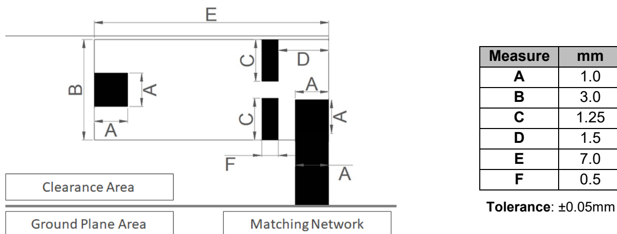
Figure 5 – Footprint dimensions for the NN03-320 in the corner for UWB.
